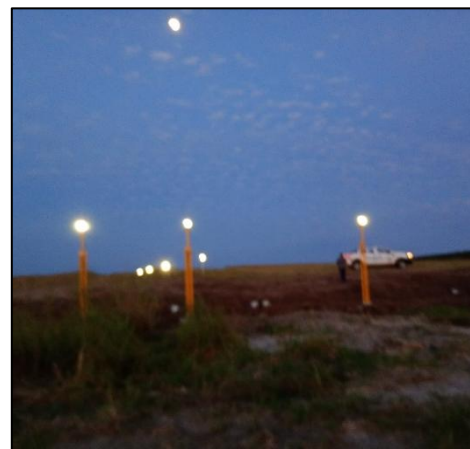
Approach lights installed
